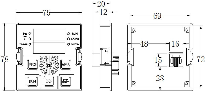
Figure 2-9.1 External dimensions of keyboard without tray (Mounting hole size 69*72)
