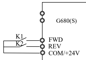
Figure3-14 Two-phase operation mode 2
