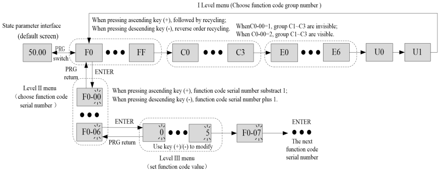
Figure 4-2. Three-level menu operation flowchart
