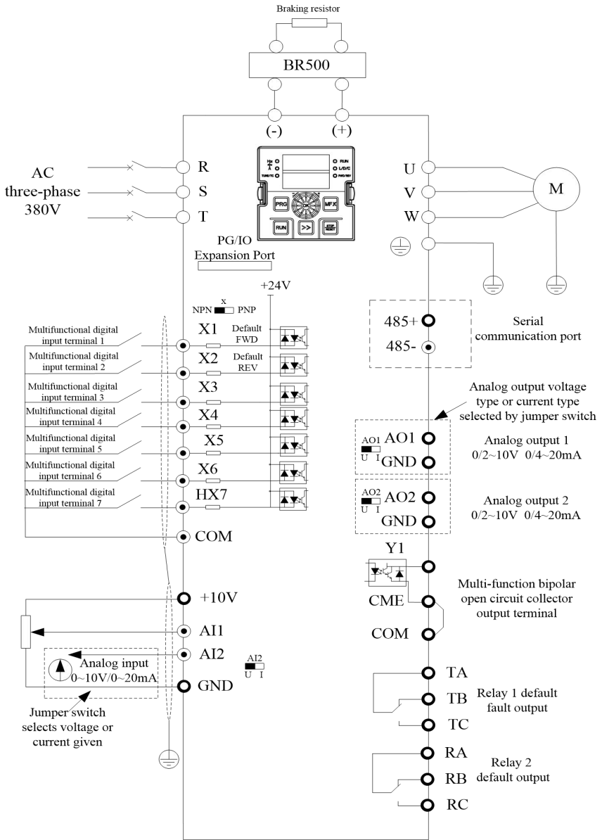
Figure 3-3. 3-phase 380V 37 ~ 75 kW (4T:380V) without brake unit function wiring diagram
