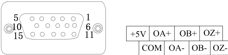
Appendix B: Figure 7 G680-PGS Terminal Diagrams
