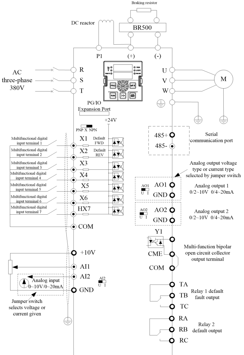
Figure 3-4. 3-Phase 380V 93kW (4T:380V) and Above 3-Phase Inverter Wiring Diagrams
