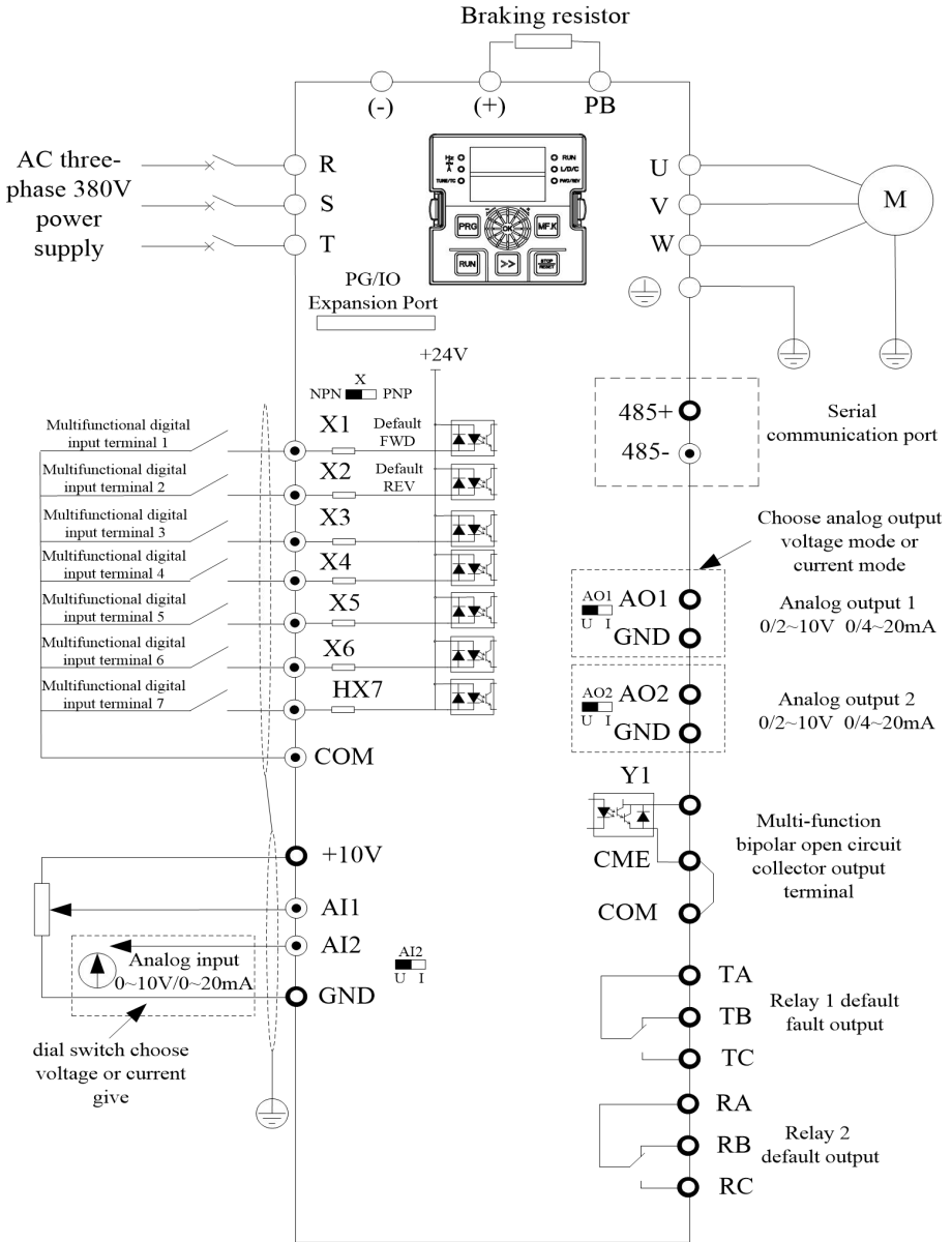
Figure 3-2. 3-phase 380V 0.75-30kW (4T:380V) and single-phase 220V (2S) 5.5kW or less (input connected to R T) Inverter Wiring Diagrams
