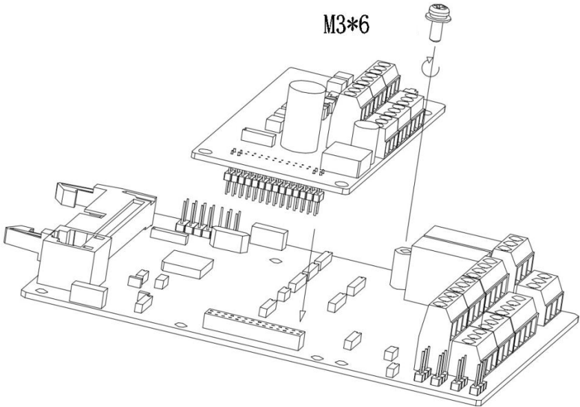
Appendix C: Figure1 G680/G680S Expansion Card Mounting Style
