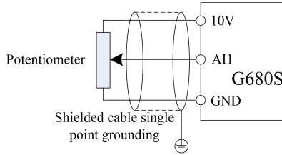
Figure 3-10. Analogue Input Terminal Wiring Schematic
