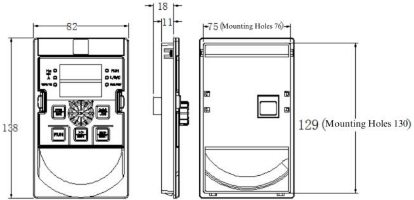
Figure 2-8.1 External dimensions of keyboard with tray (Mounting hole size 76*130)
