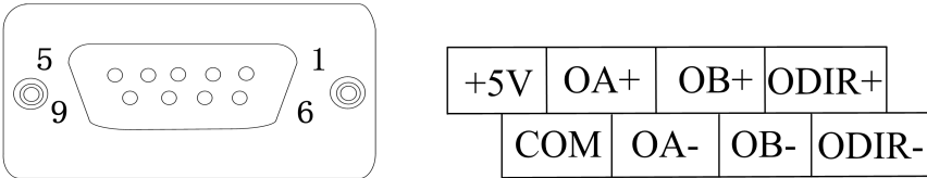
Appendix B: Figure 5 G680-PGR Terminal Diagrams
