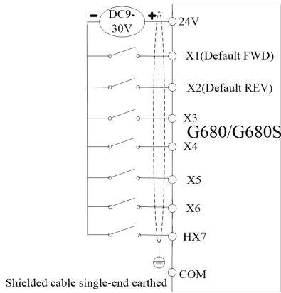
X terminal connection Mode 2: DI dial switch in NPN mode and with external power supply
